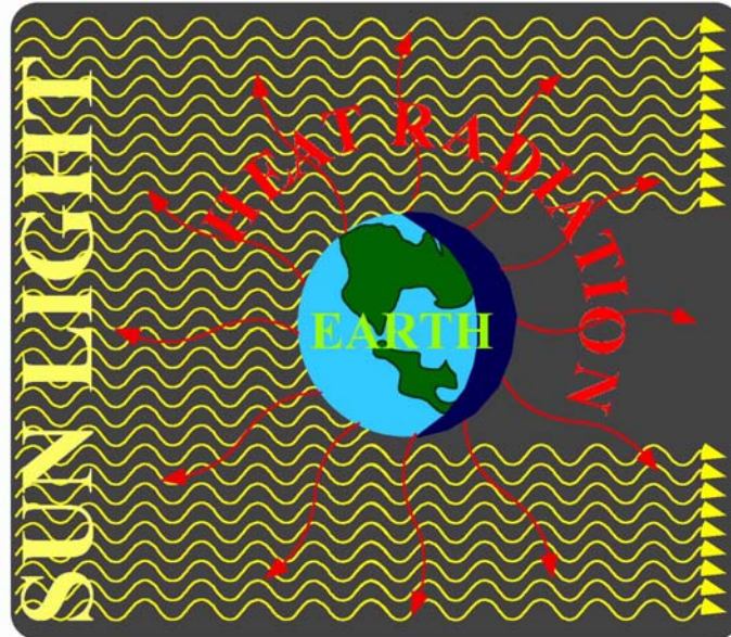
Figure 4. Short-wave sunlight inwards and long-wave heat radiation outwards.
