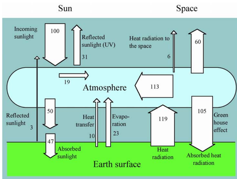
Figure 6. The energy flow between the Sun, the atmosphere, the surface of the Earth and space. Numbers are in percent of incoming sunlight.
