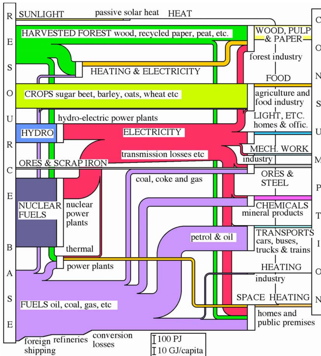
Figure 16. The exergy conversion system in the Swedish society in 1994. Total input about 2720 PJ or 310 GJ per capita and output about 380 PJ or 43 GJ per capita.
