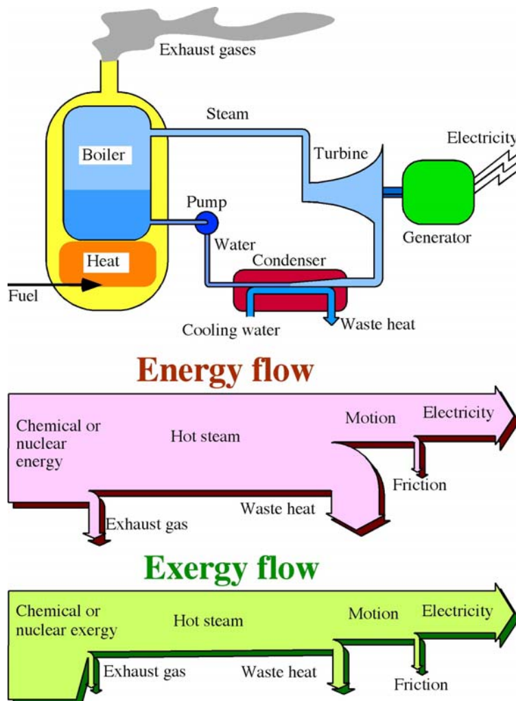
Figure 17. Energy and exergy flows through a condensing power plant.
