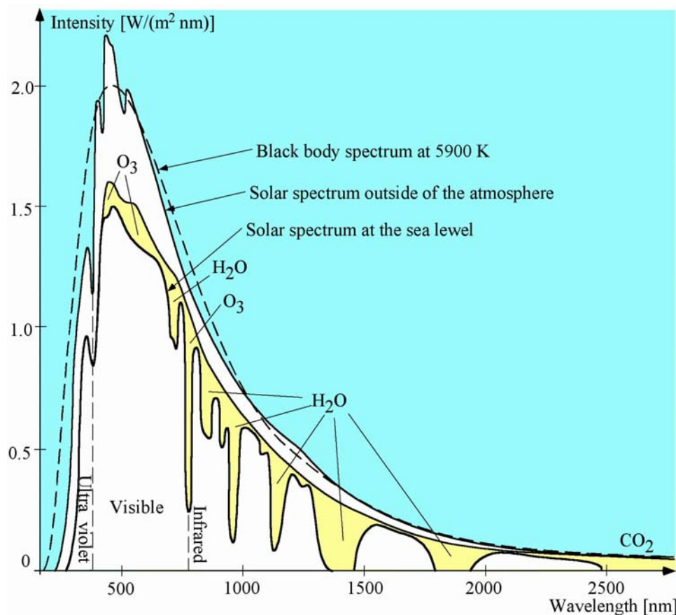
Figure 5. The intensity of sunlight at the surface of the Earth with respect to wavelength.
