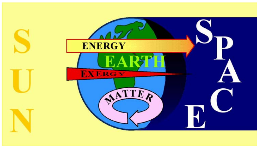
Figure 3. The Sun-Earth-space system.
