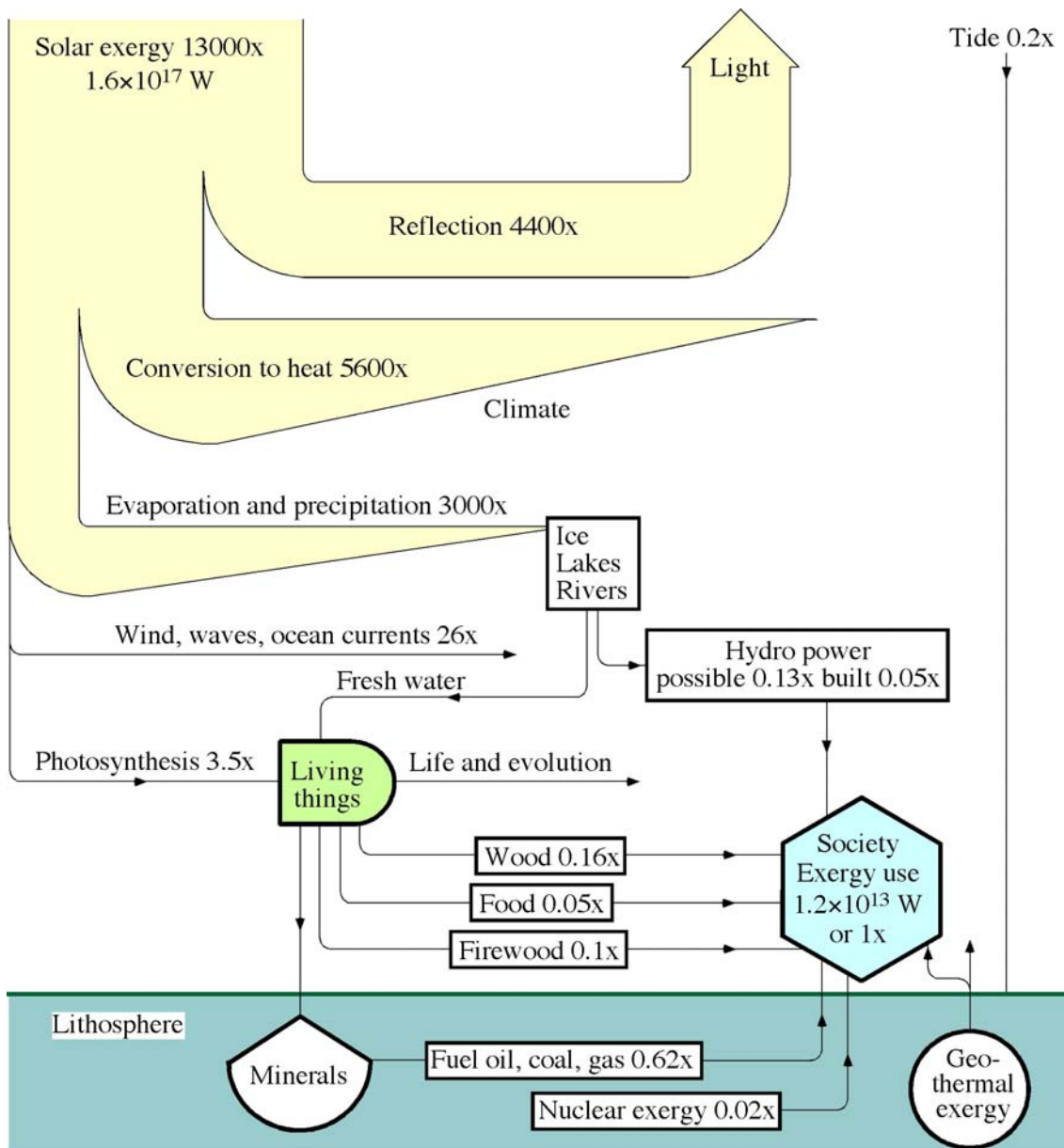
Figure 7. The global exergy flows on the Earth, where 1x is equal to 1.2 \times 10^{13} W.
