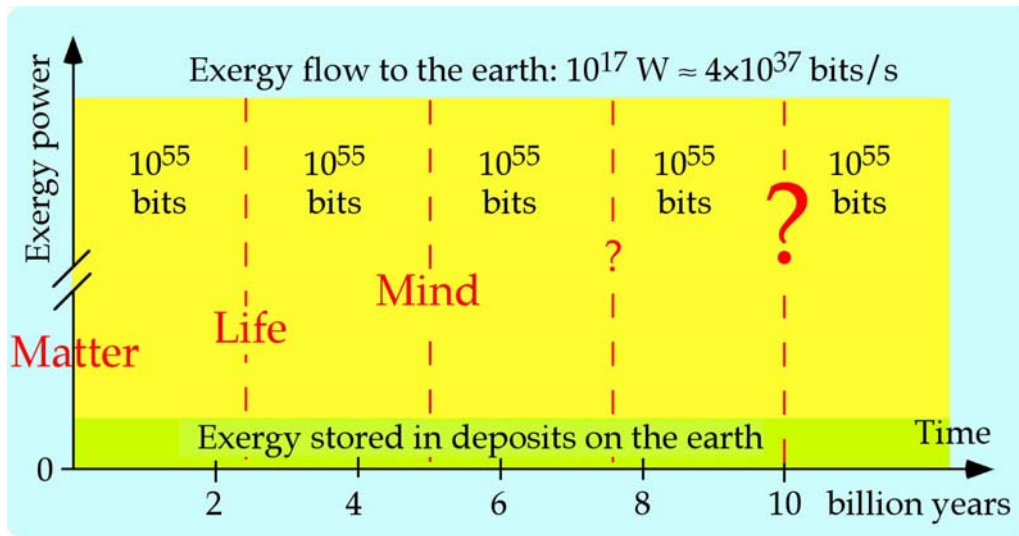
Figure 9. A tiny part of the exergy flow from the Sun to the Earth is stored in deposits on the Earth, while matter is organized into life and further into the mind, and further into ...?
