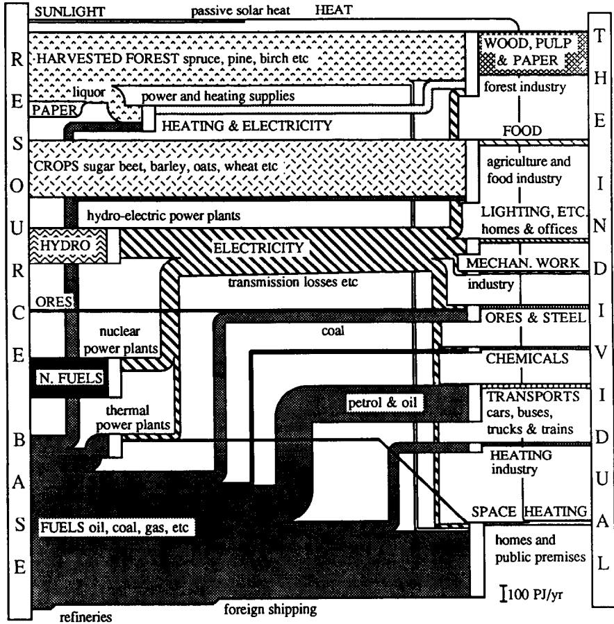
Fig. 2. The exergy conversion system in Swedish society in 1980. Total conversion 2539 PJ or 305 GJ/capita; net output 500 PJ or 60 GJ/capita.
