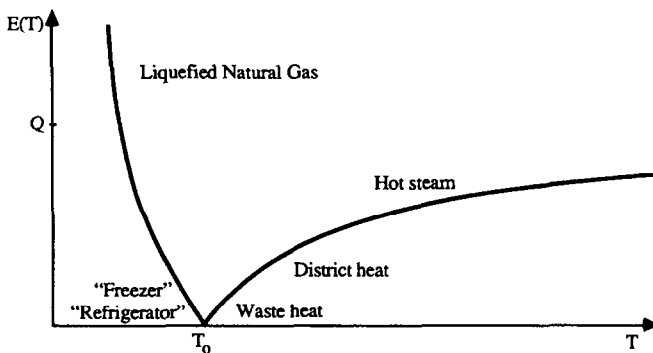
Fig. 3. Exergy as a function of temperature.
