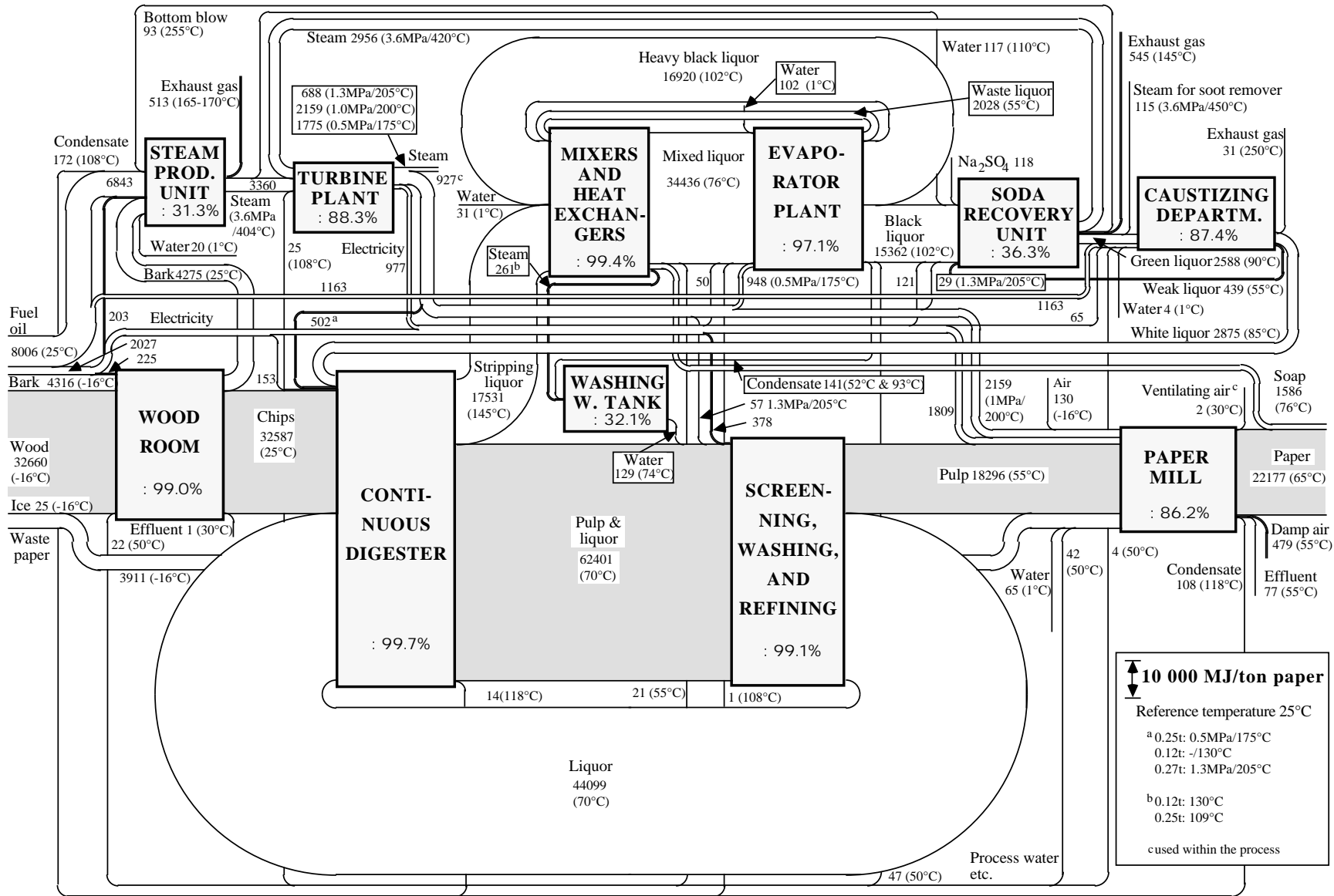
THE EXERGY FLOW IN A SWEDISH KRAFT LINER MILL (SCA-MUNKSUND) DURING JANUARY 1979
