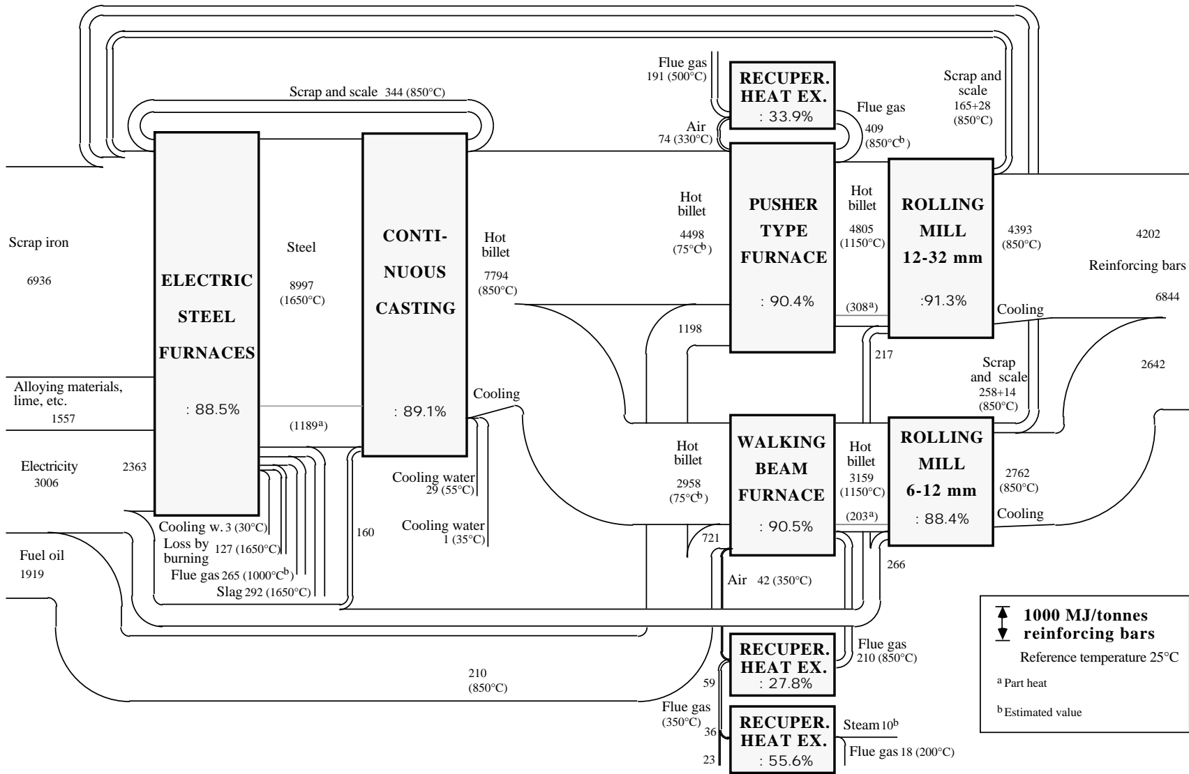
THE EXERGY FLOW IN A SWEDISH STEEL PLANT (HALMSTADS JÄRNVERK) DURING MARCH 1976
